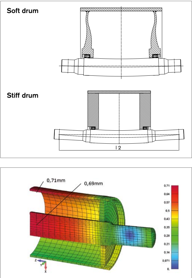
Deformation on an belt drum
